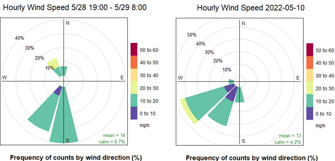
Figure 6. Wind speed and direction frequency for (left) the May 28-29, 2022, suspected exceptional event period, and (right) May 10, 2022.
