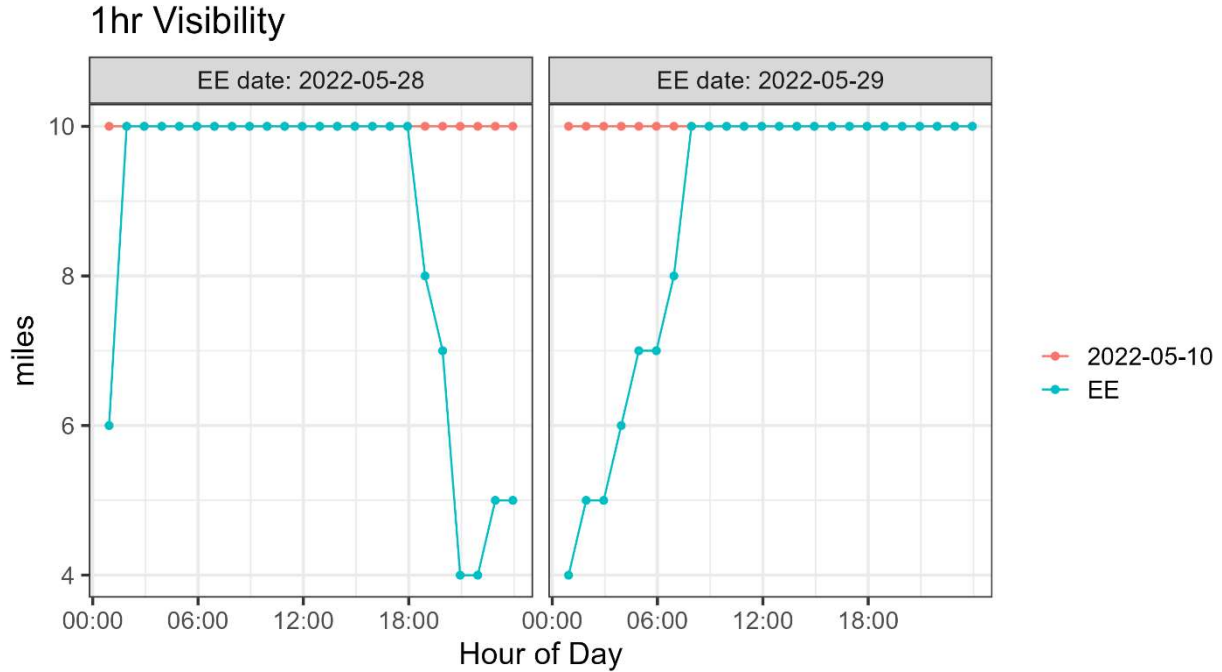
Figure 7. Hourly visibility in miles at LAS for May 10, 2022 (pink), and the May 28-29, 2022, suspected exceptional event period [EE] (teal).
