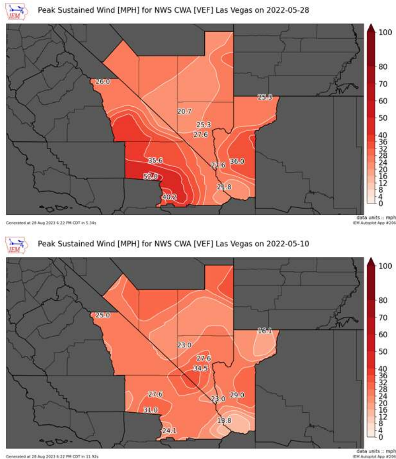
Figure 9. Spatial distribution of peak sustained wind speeds on May 28 (top) and May 10 (bottom), 2022, in Clark County and the surrounding regions. Generated from an automated ASOS data using the Iowa Environmental Mesonet’s plotter tool ( https://mesonet.agron.iastate.edu/plotting/auto ).
