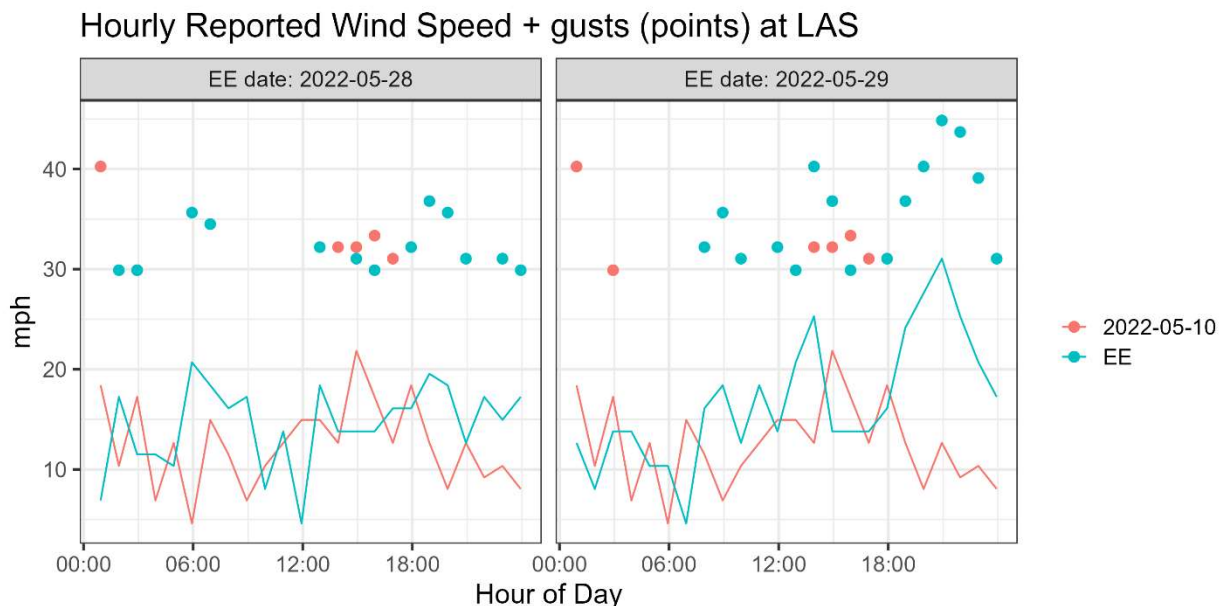
Figure 5. Wind speed and maximum hourly wind gusts in mph at LAS for May 10, 2022 (pink), and the May 28-29, 2022, suspected exceptional event [EE] period (teal).
