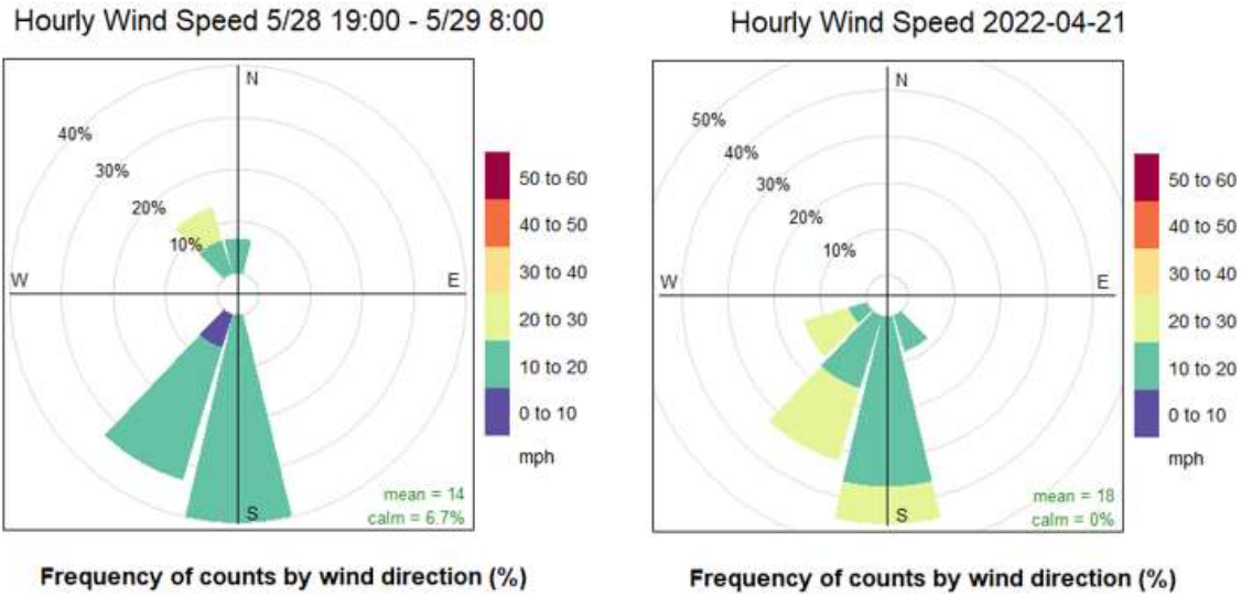
Figure 2. Wind speed and direction frequency for (left) the May 28-29, 2022, suspected exceptional event period, and (right) April 21, 2022.
