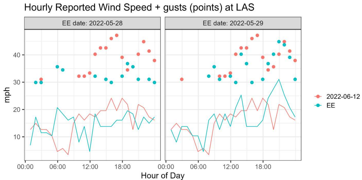
Figure 10. Wind speed and maximum hourly wind gusts in mph at LAS for June 12, 2022 (pink) and the May 28-29, 2022 suspected exceptional event [EE] period (teal).
