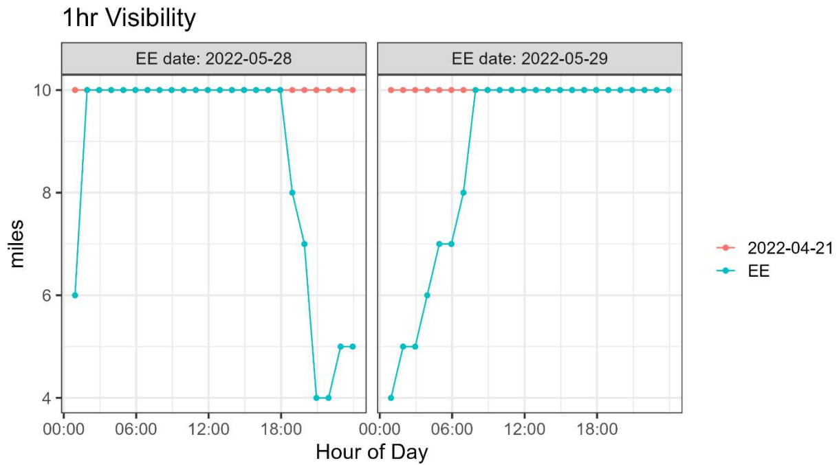
Figure 3. Hourly visibility in miles at LAS for April 21, 2022 (pink), and the May 28-29, 2022, suspected exceptional event period [EE] (teal).
