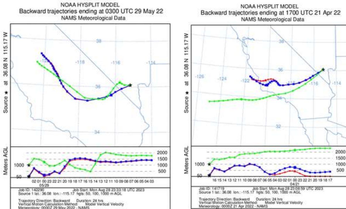
Figure 4. 24-hour HYSPLIT back-trajectories initiated from Las Vegas at (left) 03:00 UTC on May 29, 2022 (19:00 PST on May 28) (event period), and (right) 17:00 UTC on April 21, 2022 (09:00 PST), at 50 m (red), 100 m (blue) and 1,000 m (green).
