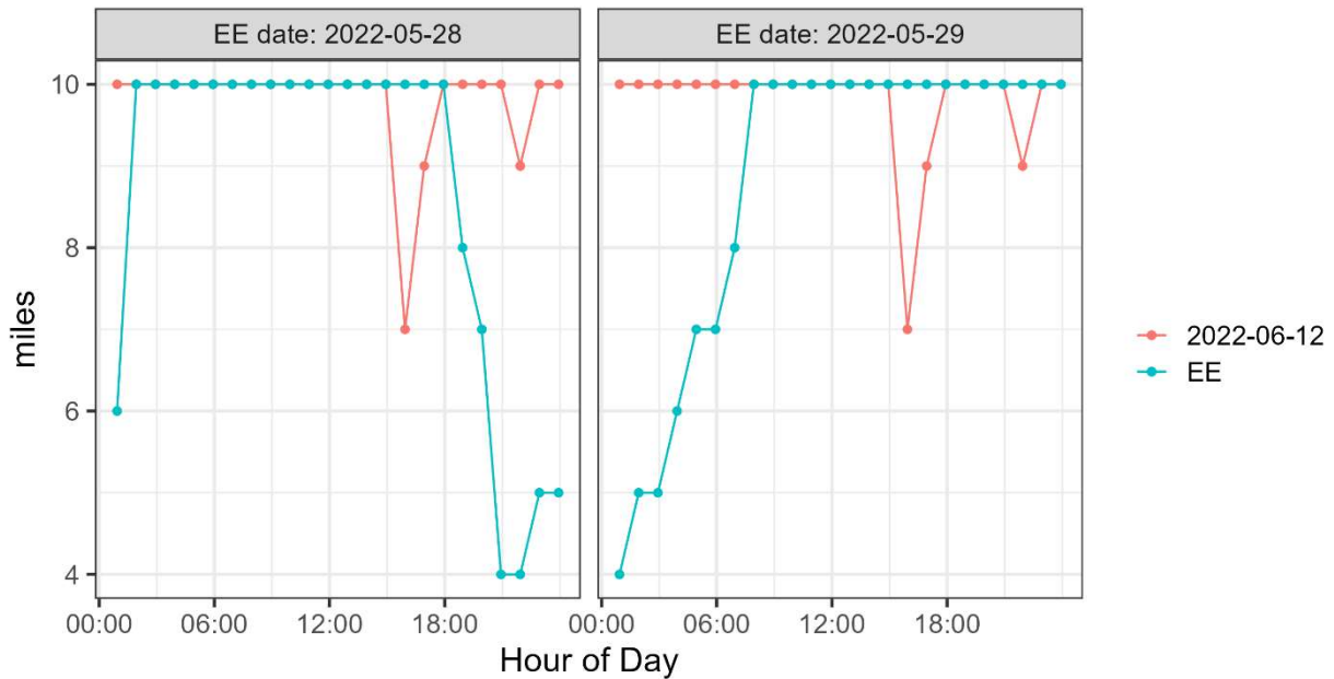
Figure 12. Hourly visibility in miles at LAS for June 12, 2022 (pink), and the May 28-29, 2022, suspected exceptional event period [EE] (teal).
