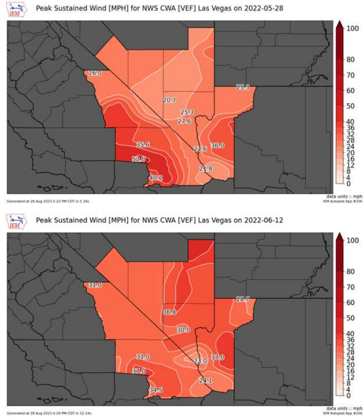
Figure 14. Spatial distribution of peak sustained wind speeds on May 28 (top) and June 12 (bottom), 2022, in Clark County and the surrounding regions. Generated from an automated ASOS data using the Iowa Environmental Mesonet's plotter tool ( https://mesonet.agron.iastate.edu/plotting/auto ).
