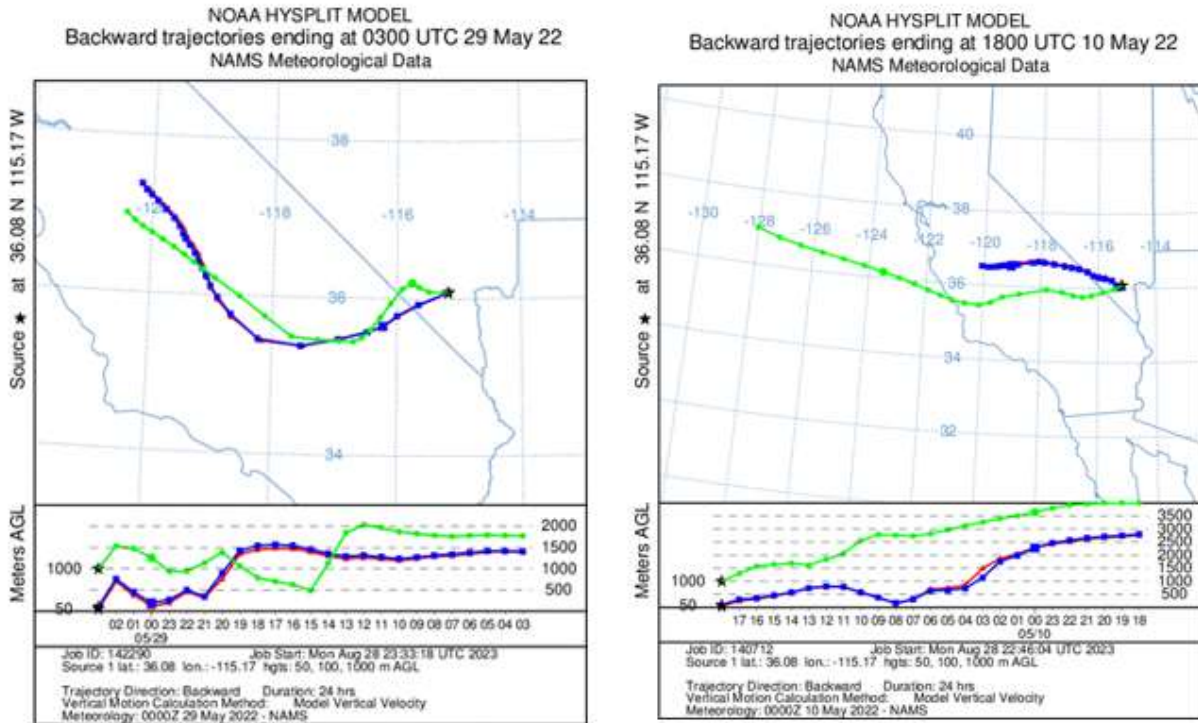
Figure 8. 24-hour HYSPLIT back-trajectories initiated from Las Vegas at (left) 03:00 UTC on May 29, 2022 (19:00 PST on May 28) (event period), and (right) 18:00 UTC on May 10, 2022 (10:00 PST) at 50 m (red), 100 m (blue) and 1,000 m (green).
