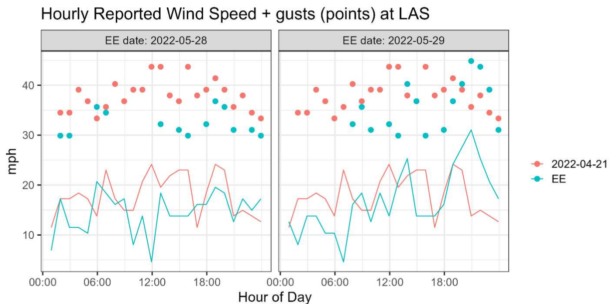
Figure 1. Wind speed and maximum hourly wind gusts in mph at LAS for April 21, 2022 (pink), and the May 28-29, 2022, suspected exceptional event [EE] period (teal).
